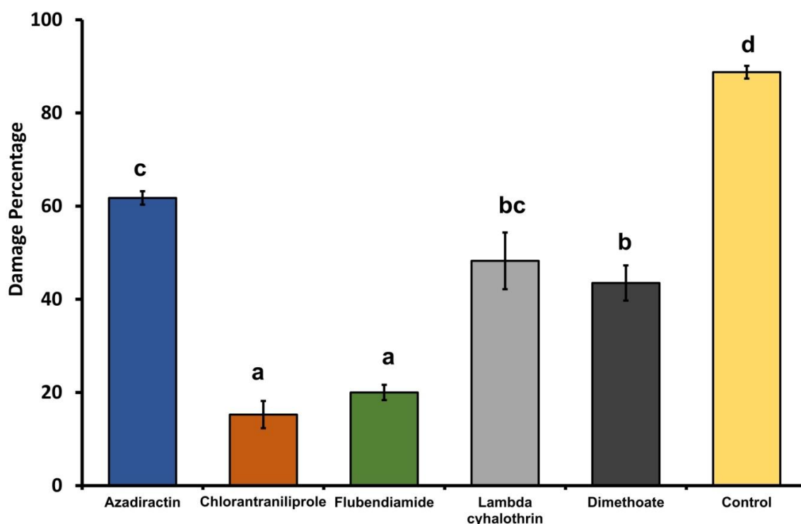
Figure 2. Mean percentage damage of Conopomorpha sinensis on Litchi in 2016 on Regional Agricultural Research Station (RARS), Tarahara, Sunsari. (Bars with same letter for each treatment represents the damage was not significantly difference at P < 0.05\% .)
